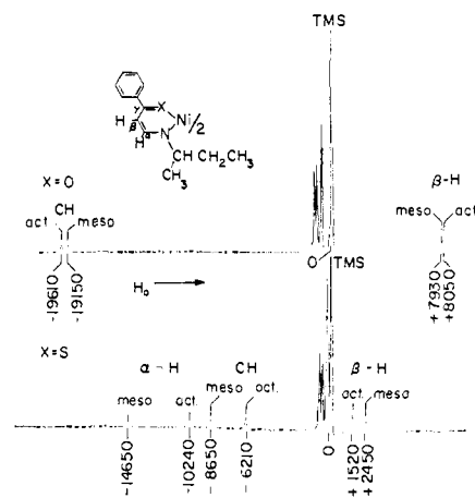
Figure 3. Pmr spectra (100 MHz) of mixtures of active and meso isomers of \text{Ni}(\text{sec-Bu-PhHH})_2 and \text{Ni}(\text{sec-Bu-SPhHH})_2 in \text{CDCl}_3 solution at \sim 30^\circ ( \alpha\text{-H} signals of the former not shown).
