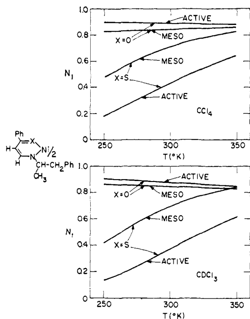
Figure 5. Temperature dependence of the tetrahedral mole fractions of the diastereoisomers of \text{Ni}(\text{Amp-PhHH})_2 and \text{Ni}(\text{Amp-SPhHH})_2 in carbon tetrachloride and chloroform solutions evaluated from data in Table VI.
