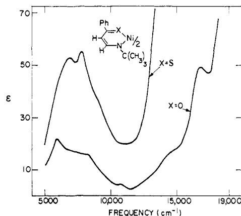
Figure 1. Electronic absorption spectra of Ni( t -Bu-PhHH) 2 and Ni( t -Bu-SPhHH) 2 in chloroform solution at 25°.
