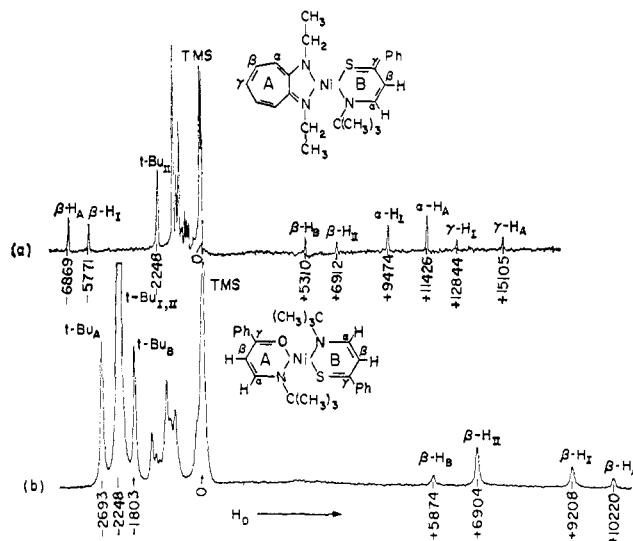
Figure 6. Pmr spectra (100 MHz) at \sim 30^\circ in \text{CDCl}_3 solution: (a) mixed ligand complex formed by \text{Ni}(\text{Et}_2\text{-ati})_2 (I) and \text{Ni}(t\text{-Bu-SPhHH})_2 (II); (b) mixed ligand complex formed by \text{Ni}(t\text{-Bu-PhHH})_2 (I) and \text{Ni}(t\text{-Bu-SPhHH})_2 (II).
