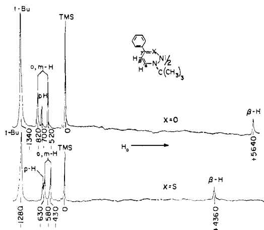
Figure 2. Pmr spectra (60 MHz) of \text{Ni}(t\text{-Bu-PhHH})_2 and \text{Ni}(t\text{-Bu-SPhHH})_2 in \text{CCl}_4 solution at \sim 30^\circ ( \alpha\text{-H} signals not shown).
