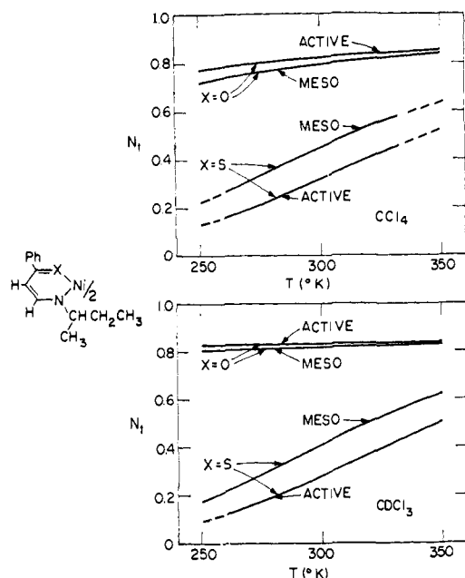
Figure 4. Temperature dependence of the tetrahedral mole fractions of the diastereoisomers of \text{Ni}(\text{sec-Bu-PhHH})_2 and \text{Ni}(\text{sec-Bu-SPhHH})_2 in carbon tetrachloride and chloroform solutions evaluated from data in Table VI.
